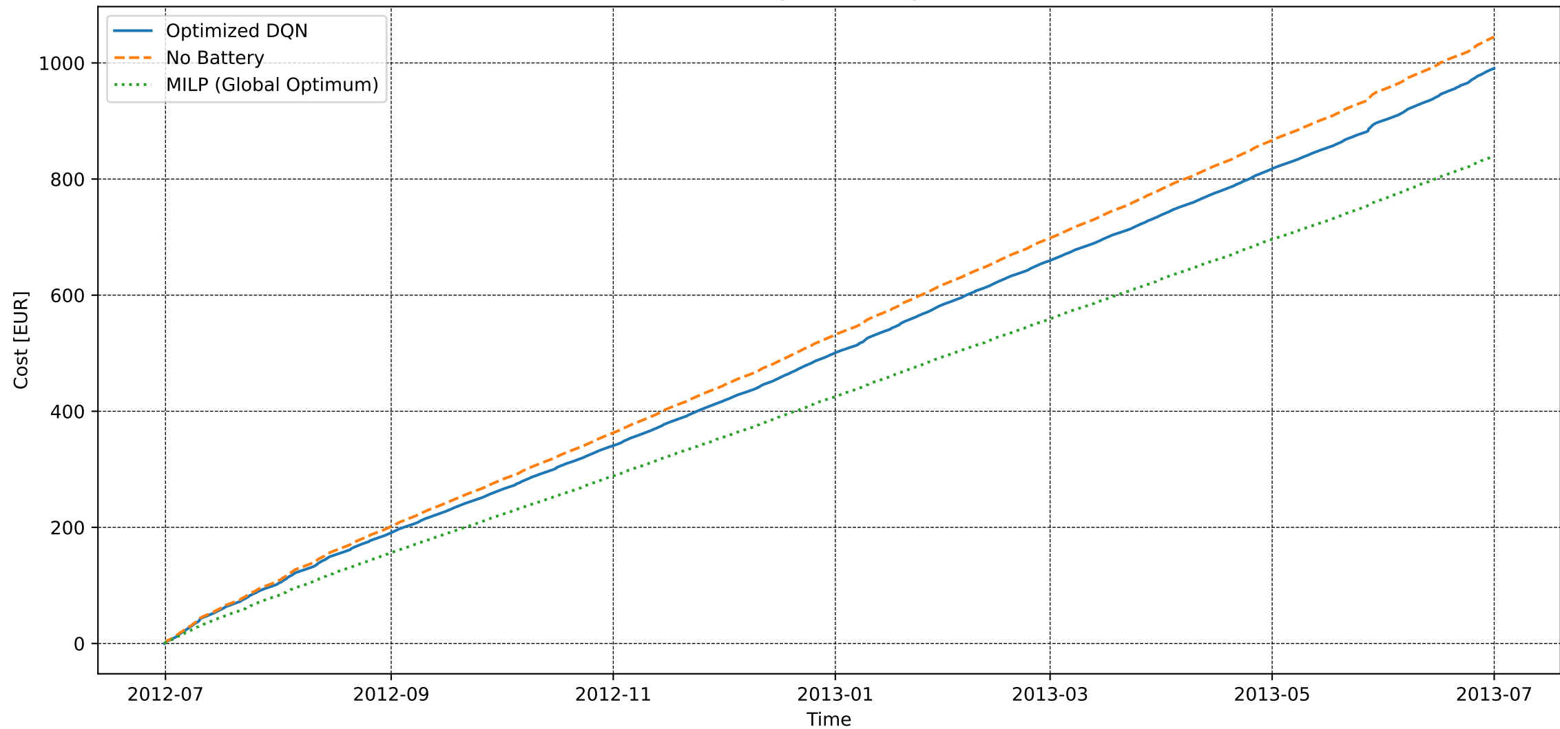
User 261 - Basic Training - Electricity Cost [DQN vs MILP]
